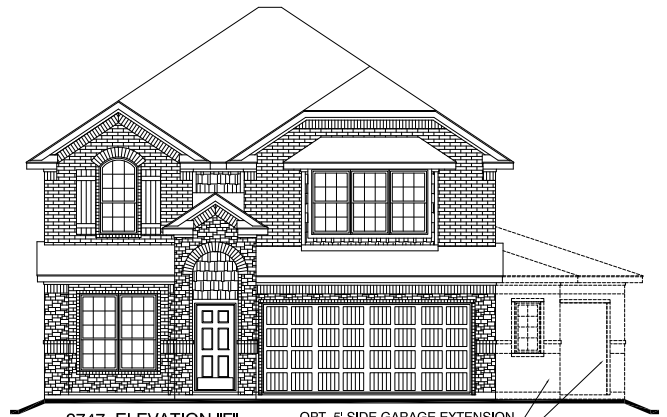
2747 ELEVATION "F" OPT. 5' SIDE GARAGE EXTENSION OPT. 3RD CAR GARAGE
