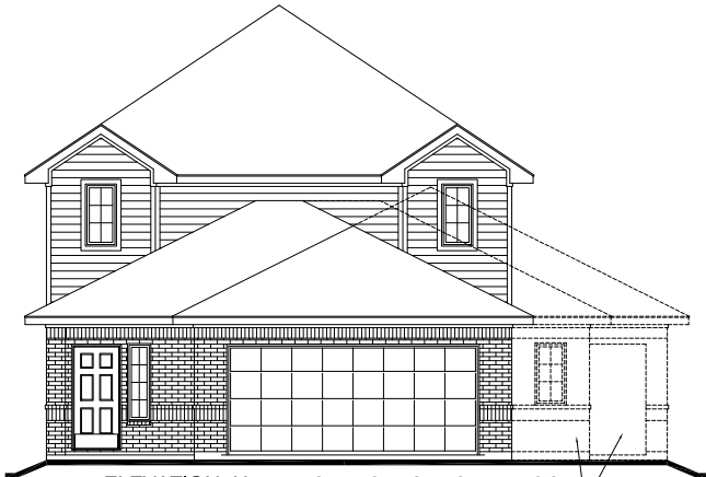
2628 ELEVATION "H" OPT. 5' SIDE GARAGE EXTENSION OPT. 3RD CAR GARAGE
