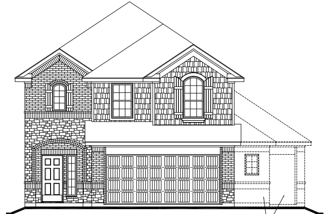
2331 ELEVATION "E" OPT. 5' SIDE GARAGE EXTENSION OPT. 3RD CAR GARAGE
