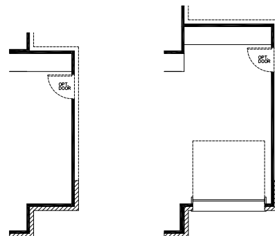
OPT. 5' SIDE GARAGE EXTENSION
