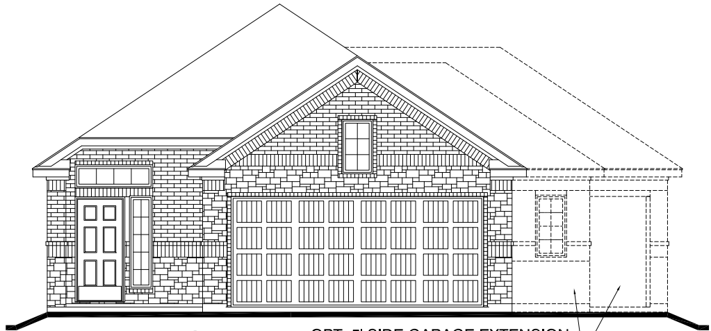
1589 ELEVATION "E"
