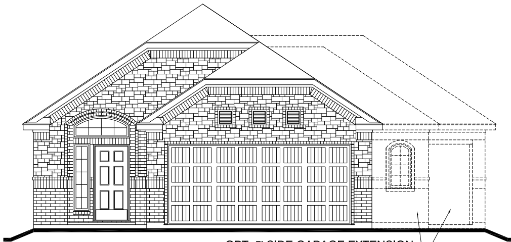
1589 ELEVATION "F"
