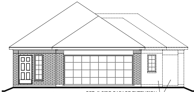
1589 ELEVATION "H" OPT. 5' SIDE GARAGE EXTENSION OPT. 3RD CAR GARAGE
