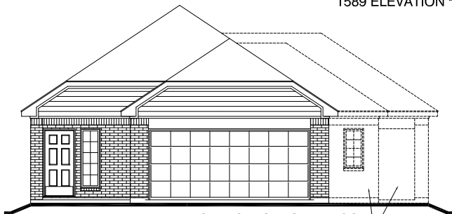
1589 ELEVATION "J" OPT. 5' SIDE GARAGE EXTENSION OPT. 3RD CAR GARAGE
