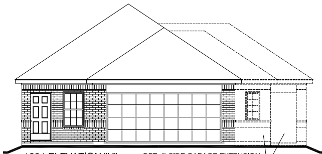
1394 ELEVATION "H" OPT. 5' SIDE GARAGE EXTENSION OPT. 3RD CAR GARAGE
