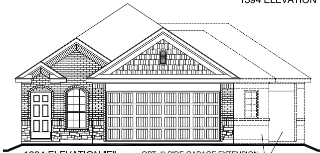
1394 ELEVATION "E" OPT. 5' SIDE GARAGE EXTENSION OPT. 3RD CAR GARAGE
