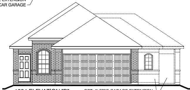
1394 ELEVATION "D" OPT. 5' SIDE GARAGE EXTENSION OPT. 3RD CAR GARAGE
